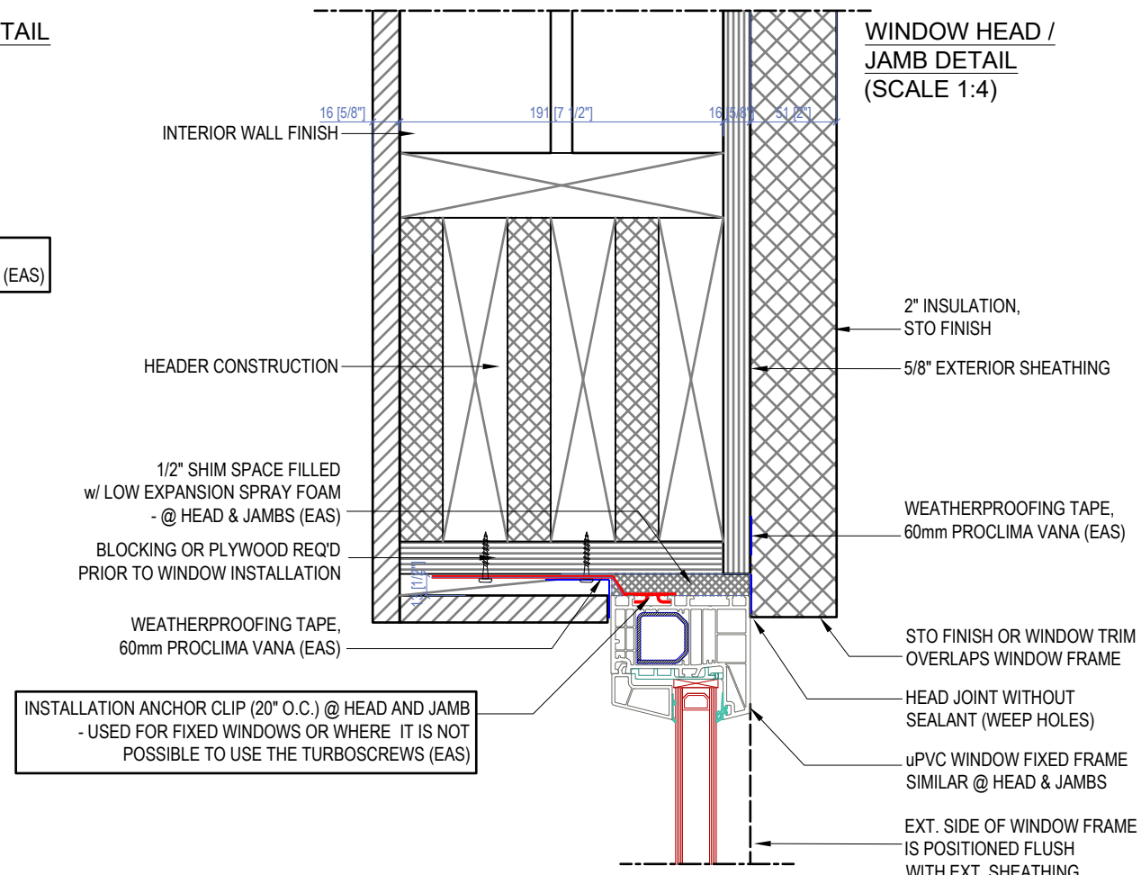
uPVC FIXED WINDOW CLIP INSTALLATION
