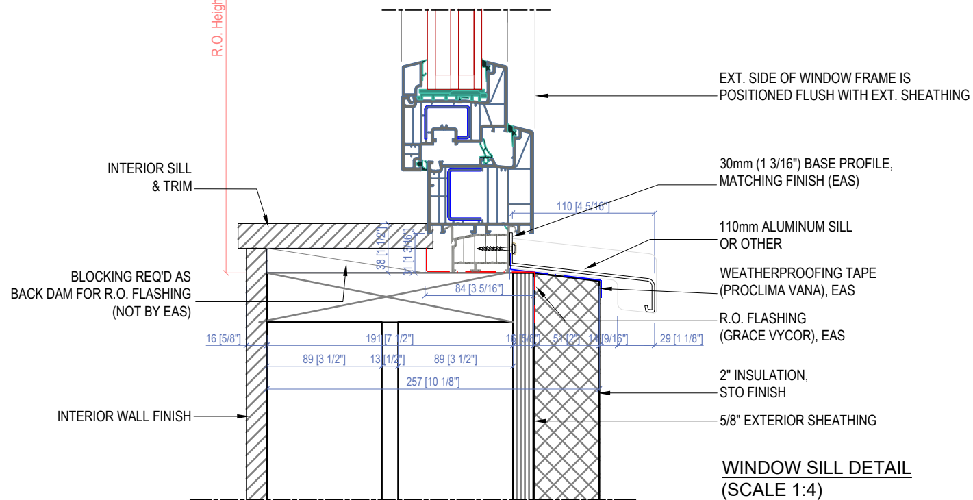
uPVC OPERABLE WINDOW TURBO-SCREW INSTALLATION
